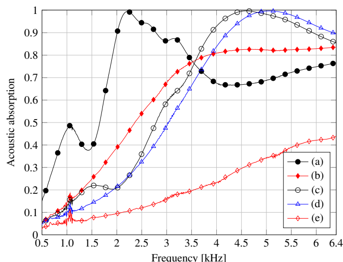
Figure 10: Acoustic absorption of a polyurethane foam of single, microscopic porosity: (a) a clean sample, 16 mm-thick, (b) the 16 mm-thick sample coated with MR fluid and exposed to a magnetic field, (c) a clean sample, 7 mm-thick, (d) the 7 mm-thick sample coated with MR fluid (no magnet), (e) the 7 mm-thick MR fluid-coated sample in magnetic field.
