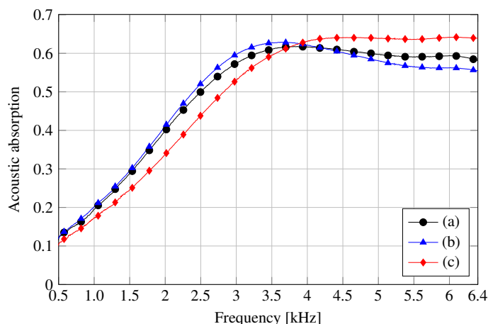
Figure 8: Acoustic absorption of a stiffer foam of single, microscopic porosity: (a) a clean sample, (b) samples with MR-coating (no magnet), (c) the MR fluid-coated samples in magnetic field.
