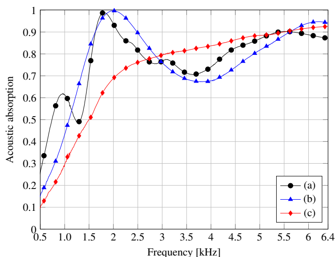
Figure 9: Acoustic absorption of a polyurethane foam of single, microscopic porosity: (a) a clean sample, 21 mm-thick, (b) the same sample with MR-coating (no magnet), (c) the MR fluid-coated sample in magnetic field.
