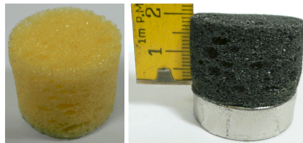
Figure 4: A 21 mm-thick sample of polyurethane foam of dual porosity: clean (left), and MR fluid-coated and placed on a magnet (right).
