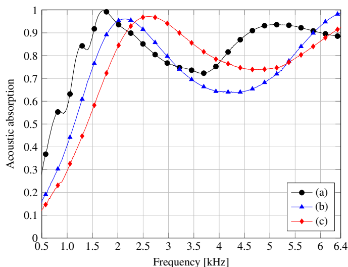
Figure 7: Acoustic absorption coefficient for polyurethane foam of dual porosity, sample B: (a) clean, (b) MR fluid-coated, (c) MR fluid-coated and exposed to a magnetic field.
