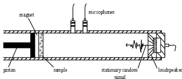
Figure 1: Diagram of an impedance tube with a magnet installed.
