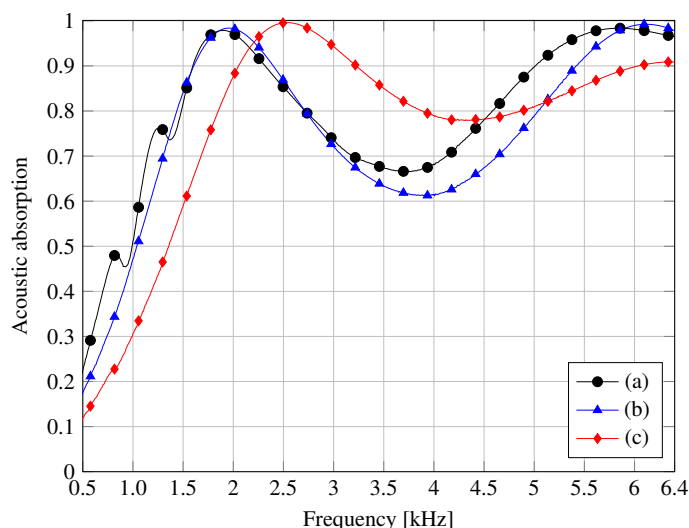
Figure 6: Acoustic absorption coefficient for polyurethane foam of dual porosity, sample A: (a) clean, (b) MR fluid-coated, (c) MR fluid-coated and exposed to a magnetic field.
