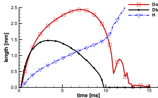
Fig. 2. Time history of the bubble equivalent diameter D_0 (squares), base diameter D_b (circles) and height H of the bubble centre of mass evaluated from the sequence of 86 images of the experiment shown in Figure 1
