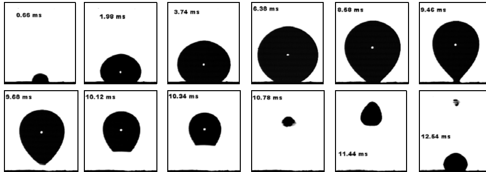
Fig. 1. Growth process of a vapour bubble (water P = 4 kPa, T_1 = 25.1^\circ\text{C} , T_s = 21.7^\circ\text{C} ) observed at 4500 frames/s by high speed camera. Frames shown at few selected time steps. Bubbles are generated at the hot spot of 1.42 mm diameter. The frame width corresponds to 2.9 mm
