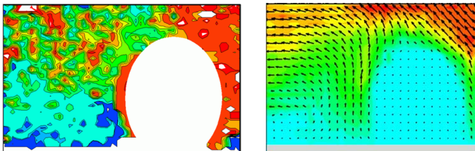
Fig. 5. Vapour bubble of water growing at the heated surface: P = 5.3 kPa, T_1 = 35.5^\circ\text{C} , T_b = 66.5^\circ\text{C} . Evaluated temperature field (left) varies from 35 - 37.5^\circ\text{C} , PIV evaluated velocity (right) has maximum magnitude 3 mm/s
