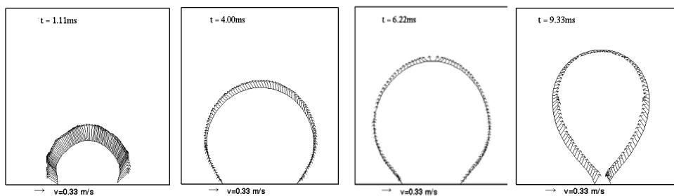
Fig. 3. PIV evaluated velocity at the bubble edge. Computations are performed considering two consecutive frames taken at the time interval 0.22 ms
