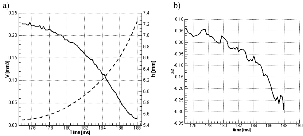
Fig. 4. Methyl alcohol vapour bubble departing from the heated surface under atmospheric pressure: a – volume (solid line) and vertical position of the bubble (dashed line); b – deformation parameter a_2 .
