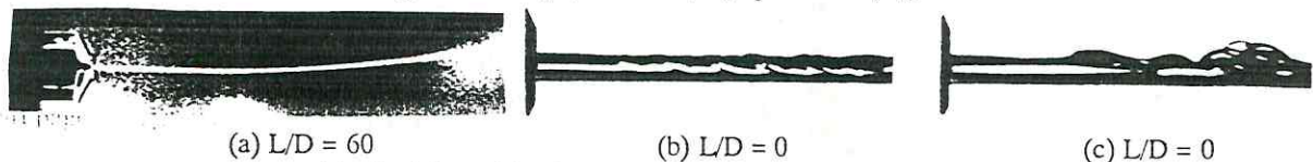
Fig. 5 - Ethanol jet, D = 200 \mu\text{m} , V = 12 \text{ m/s} , P_\infty = 5 \text{ kPa} , P_s = 5.9 \text{ kPa}
