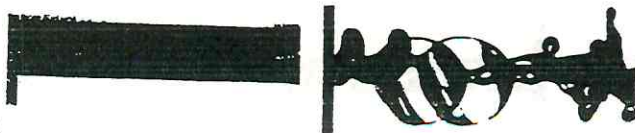
(a) L/D = 2 (b) L/D = 120 Fig. 7 - Ethanol jet, D = 200 \mu\text{m} , V = 12 \text{ m/s} , P_\infty = 5 \text{ kPa} , P_s = 5.9 \text{ kPa}
