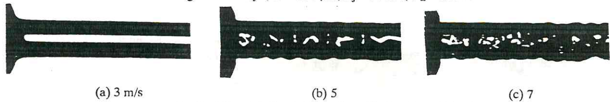
Fig. 4 - Ether jet, D = 400 \mu\text{m} , P_s = 58 \text{ kPa} , P_\infty = 100 \text{ kPa}
