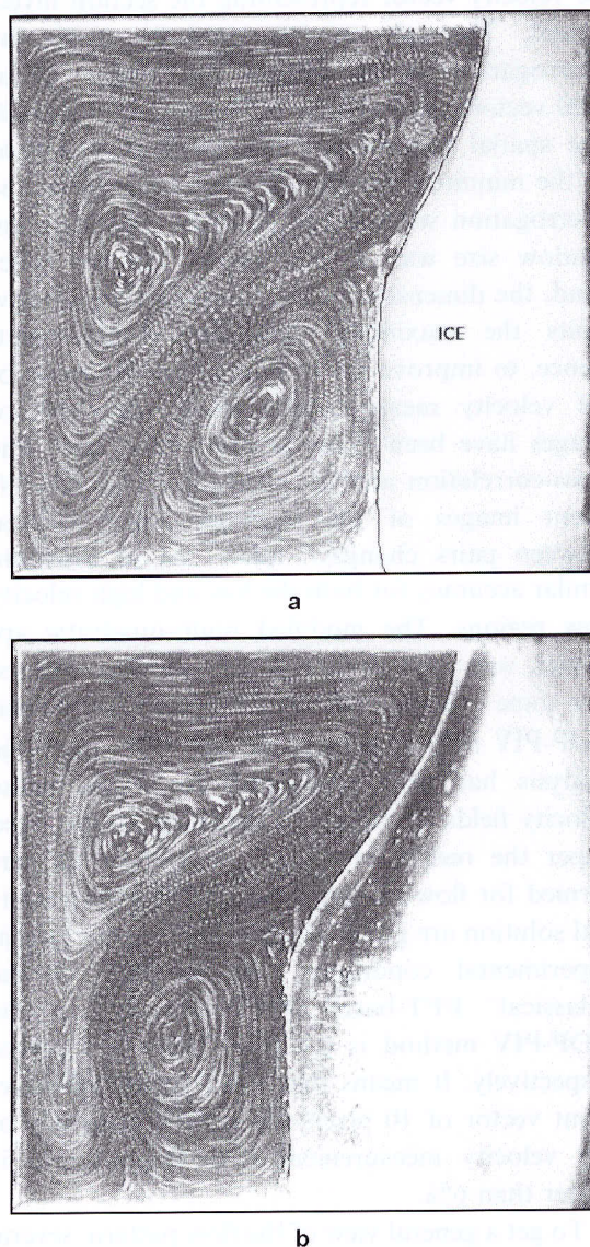
FIGURE 5 Ice fronts observed for the run #1 at 2340 s (a) and 6000 s (b) after cooling starts. Superposition of 10 images taken every 0.4 s.
