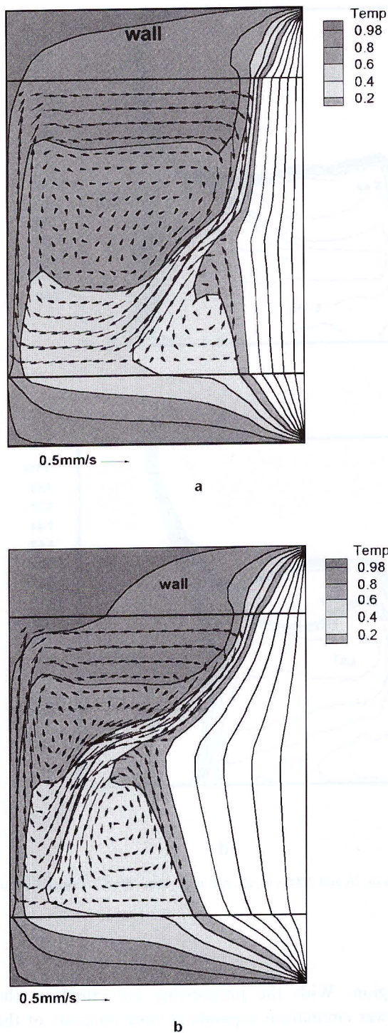
FIGURE 11 Calculated velocity and temperature fields using 3-D TBC, "warm start", external water bath; time step 500s (a) and 2600s (b). (See Color Plate III at the end of this issue.)
