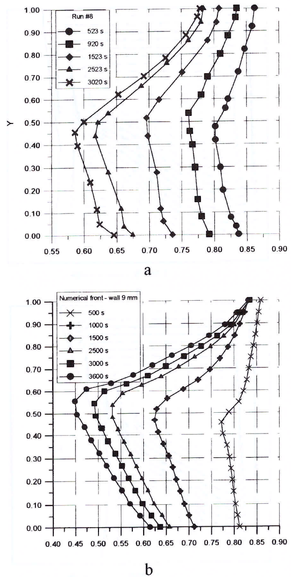
FIGURE 12 Interface profiles at selected time steps, for external fluid water, "warm start"; (a) - measured (run #8), (b) - calculated using 3-D TBC.
