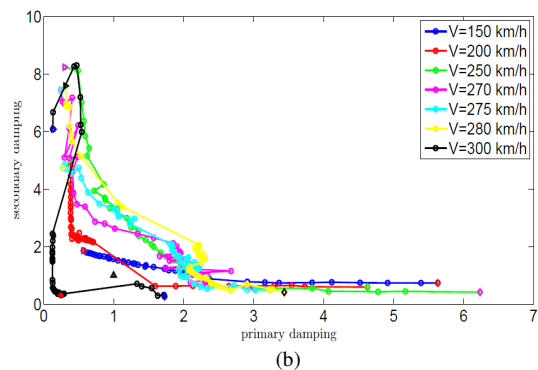
Fig. 1 Normalized Pareto fronts (a) and Pareto sets (b)
