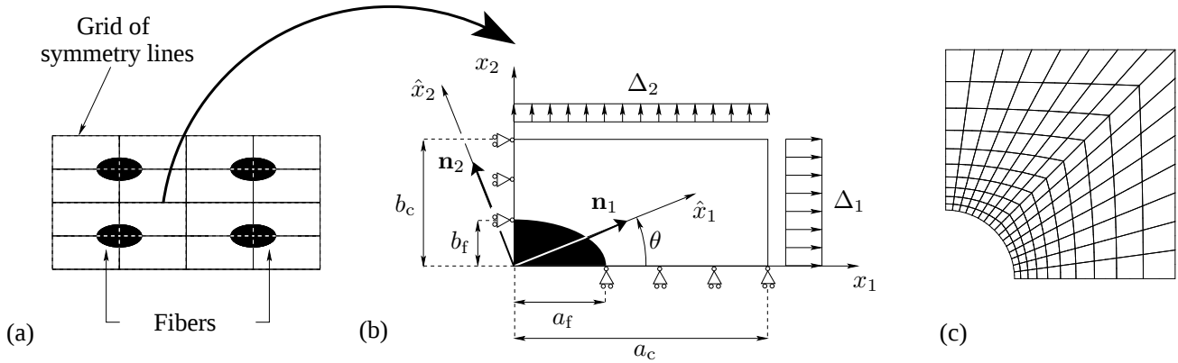
Figure 1. The plane strain cell model for the composite. (a) Periodically distributed fibers. (b) The cell used for modeling with initial dimensions, loads, supports and coordinate systems. (c) Example of finite element mesh using adopted, \frac{a_f}{b_f} = \frac{a_c}{b_c} = 1 .
