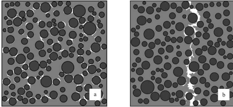
Figure 2. Effect of 'quantum' damage evolution under hydrostatic compression \varepsilon_{11}^* = \varepsilon_{22}^* = -\varepsilon_{33}^* , \varepsilon_{33}^* > 0 (a) and macrofailure of glass-epoxy plastic with fibre void fraction v_f = 0.4 under antiplane shear \varepsilon_{13}^* > 0 (b)
