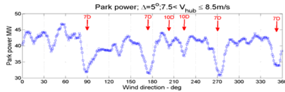
Figure 4: Power production for a wind farm at 8 m/s as function of flow direction.
