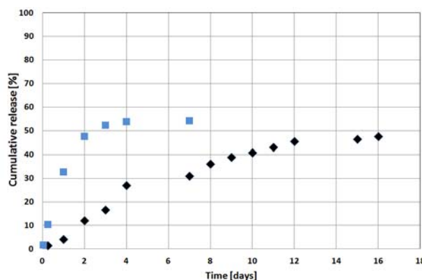
Figure 6. Cumulative release of alpha tocopherol 12 wt% from 9 wt% PLC nanofibre mat. Blue markers – mixing of supernatant during drug release, black markers – release of drug without mixing.
