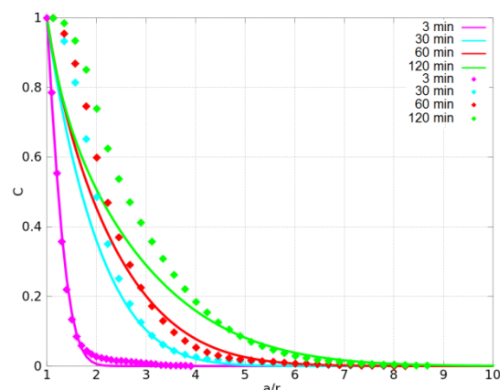
Figure 4. Dimensionless concentration – distance profiles for core-shell nanofibre. The measured data (points) and the fitted analytical model (lines). Apparent diffusion coefficient is D = 0.6 \times 10^{-11} \text{ m}^2/\text{s} .
