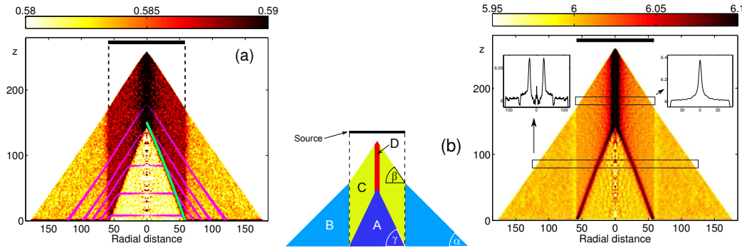
Figure 1. (a) Packing fraction for a heap with five contours superimposed showing the growth history and that the flat horizontal surface decreases as the growth proceeds. The green line segment on the right of the inner triangle shows the prediction of Eq. (1). Here N = 10^7 . (b) Schematic representation of a generic heap structure and its main characteristics: the angles of repose \alpha, \beta, \gamma , and the four characteristic density zones denoted by A..D. (c) The average contact numbers inside of the heap as a function from radial distance from the heap axis. The insets display the variation of contact numbers along the two rectangles, as indicated. Here N = 10^7 .
