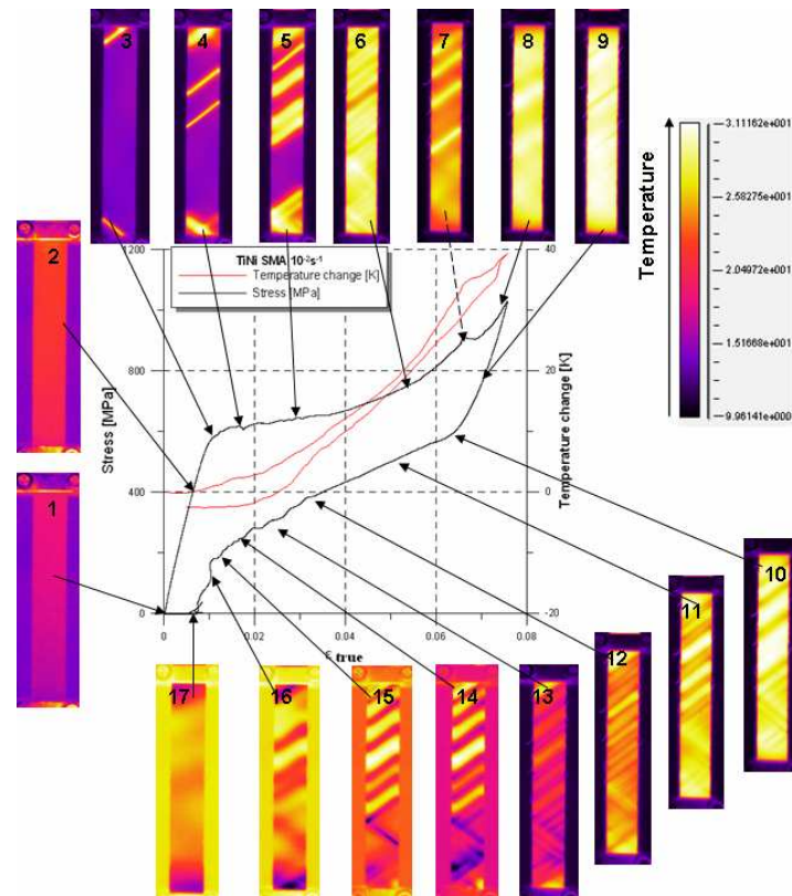
Fig. 2. Stress and temperature changes vs. strain curves obtained for TiNi SMA specimen during tension at strain rate 10^{-2}\text{s}^{-1} . Thermograms show in infrared a nucleation and evolution of macroscopic transformation bands, related to martensite forward and reverse transformation.
