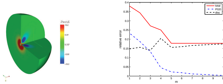
Figure 2. Example of 3D Green's function (left) and convergence of error sources with respect to PGD order m (right).
