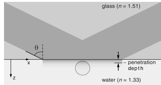
Fig. 3: Graphical representation of evanescent wave illumination.
