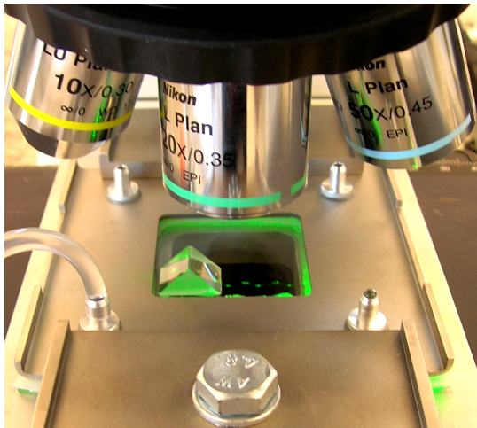
Fig. 5: Experimental channel for measurements of diffusion near the upper channel wall. Green spots are places of evanescent light reflections.
