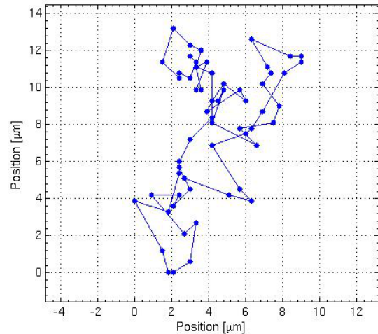
Fig. 4: Typical trajectory of a Brownian motion. The particle was 300nm in diameter, time between points is 0.5s
