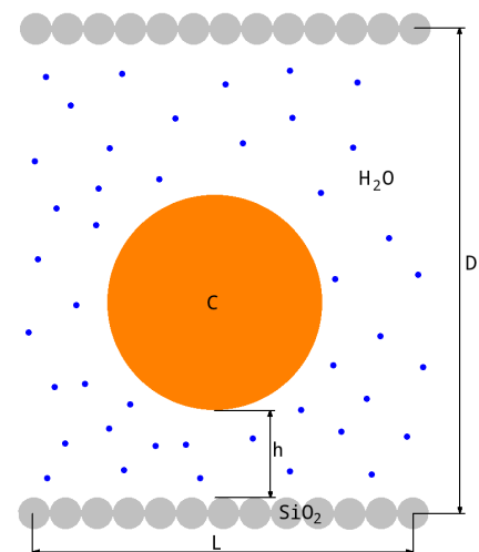
Fig. 2: MD simulation domain (not to scale) with one 24nm colloidal carbon particle suspended in water between two quartz walls. L=D=310.5\text{nm} .
