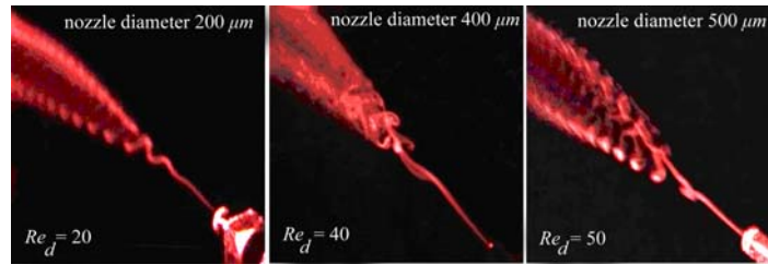
Figure 2: Smoke visualization of the micro - jet development in the transverse acoustic field with the frequency f = 200 \text{ Hz} at various diameters of the nozzle outlet orifice ( d = 200, 400, \text{ and } 500 \mu\text{m} ).
