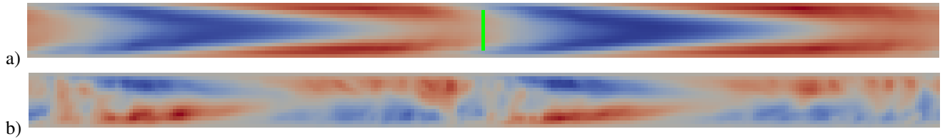
Figure 2. Mean flow \left( \int_{t=13\,000}^{15\,000} dt \int_{x=0}^{L_x} dx \right) of turbulent-laminar banded state in the (z, y) plane at Reynolds number 1400.
