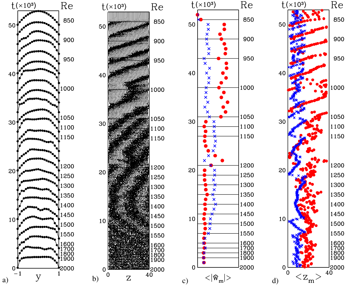
Figure 1. Simulation of plane Poiseuille flow in a domain of size L_x \times L_y \times L_z = 10 \times 2 \times 40 in which the z direction is aligned along the pattern wavevector. The Reynolds number is lowered from 2000 to 850 in discrete steps as indicated along right edge.
