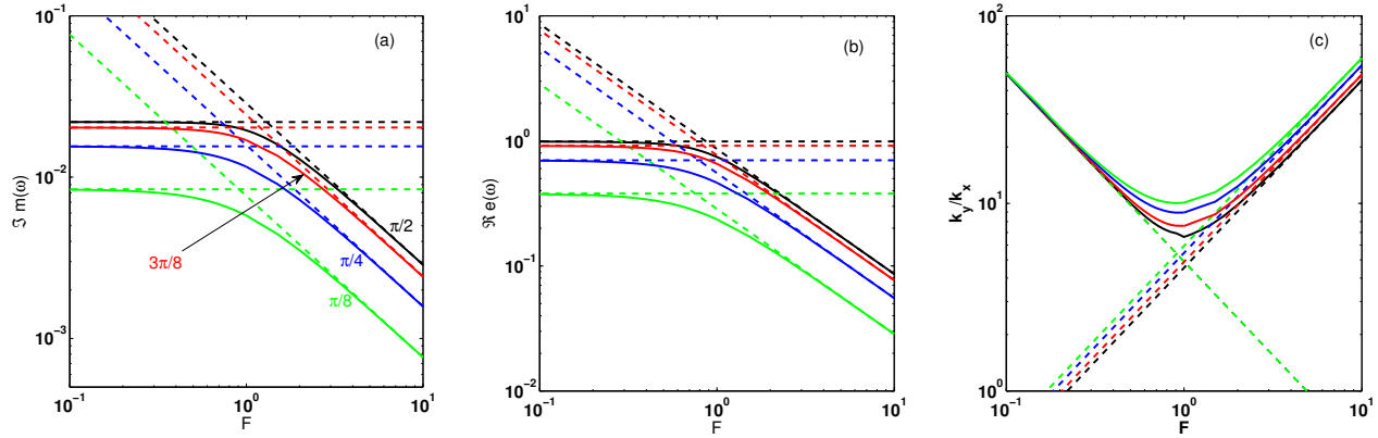
Figure 2. Characteristics of the most unstable mode over all k_y/k_x as a function of F for \theta = \pi/8, \pi/4, 3\pi/8, \pi/2 . (a) Maximum growth rate \Im m(\omega) . (b) Frequency \Re(\omega) . (c) Maximizing ratio k_y/k_x . The dotted lines are the predictions obtained from small and large F analyses.
