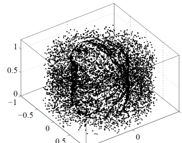
Figure 6: Instantaneous positions of bubbles ( Re=8000 \eta=0.5 ).
