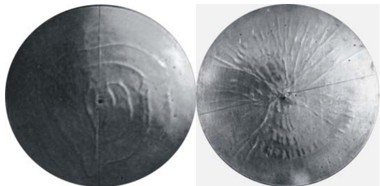
Fig.2. Secondary flows over the heater.
