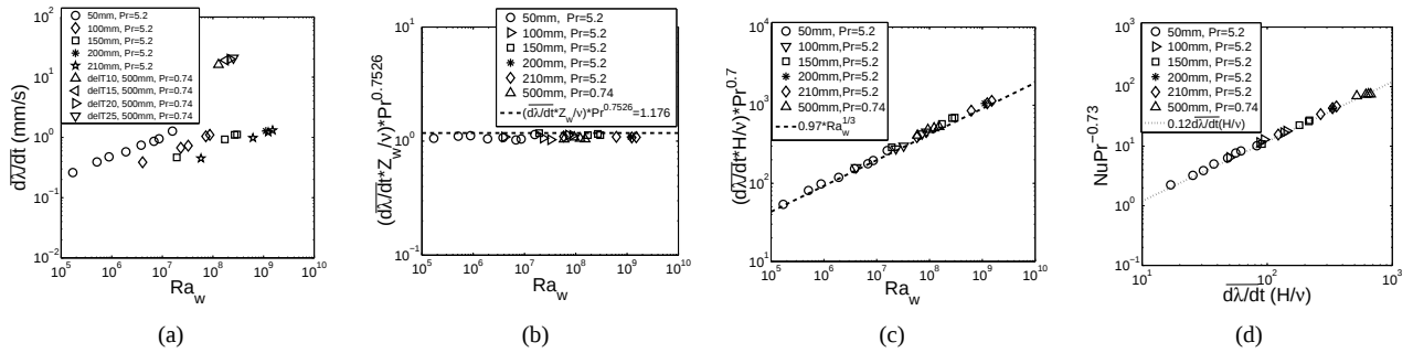
Figure 2. (a) Variation of mean velocities of merging of plumes with Ra_w for Pr = 0.74 and 5.2 (b) Variation of dimensionless mean merging velocities \bar{V}_m with the near-wall Ra_w for Pr = 0.74 and 5.2 (c) Variation of Reynolds number Re_H with Ra_w (d) Dependence of Nusselt number Nu on Re_H
