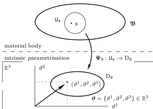
Fig. 3. Manifolds and coordinate systems
