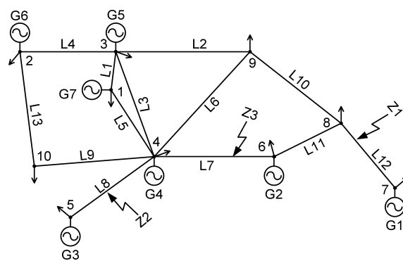
Fig. 3. CIGRE power system
