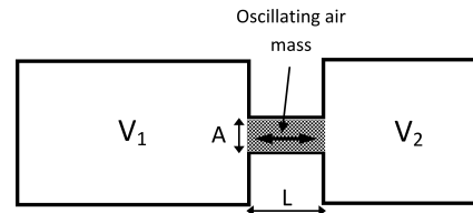
Fig. 5. The two-chamber Helmholtz resonator
