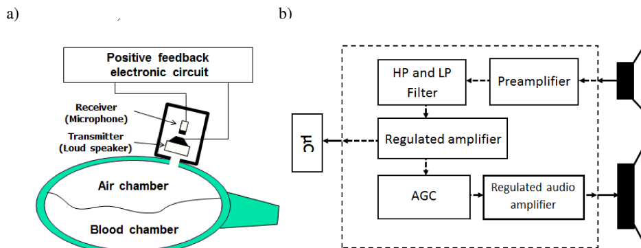
Fig. 6. The overall construction (a) and electronic circuit diagram (b) of the acoustic blood volume measurement system
