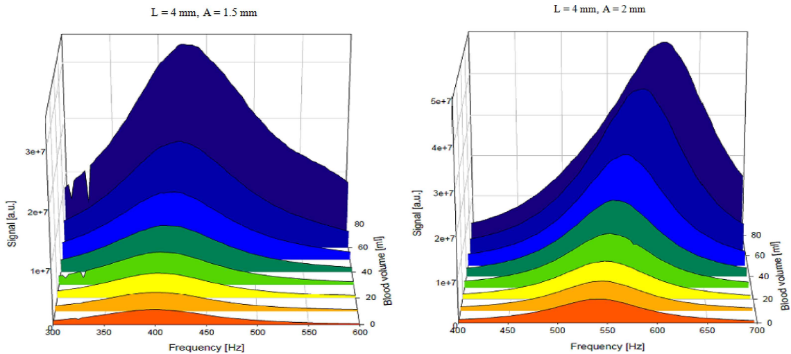
Fig. 7. Frequency characteristics of the Helmholtz resonator measurement system for different air chamber volumes
