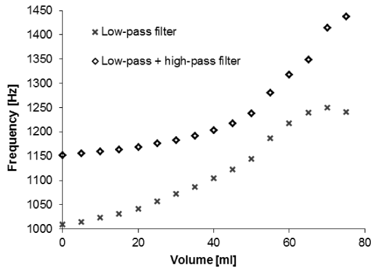
Fig. 10. Static characteristics of a new construction of the sensing system with and without the high-pass filter
