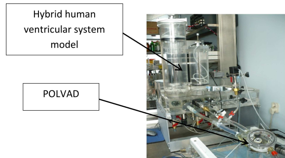
Fig. 11. Hybrid human ventricular system model for testing the POLVAD prosthesis
