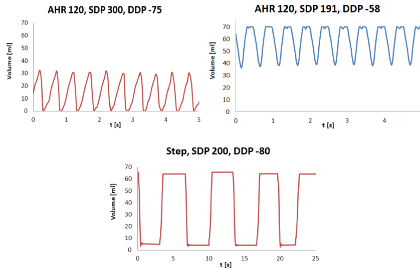
Fig. 12. Exemplary results of dynamics tests conducted at the Foundation for Cardiac Surgery Development in Zabrze
