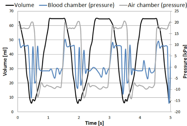
Fig. 13. The results of measurements of the acoustic sensor vs. the pressures inside the prosthesis
