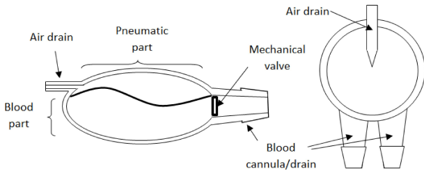
Fig. 3. Polish heart supporting device – POLVAD diagram
