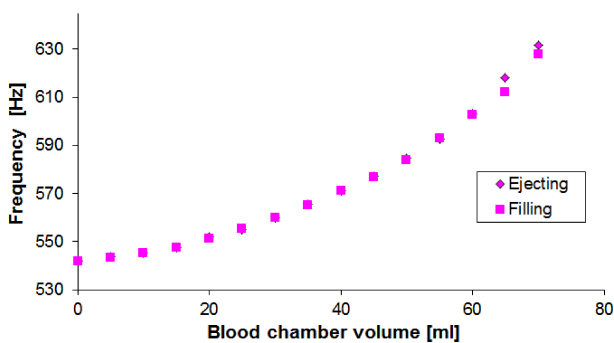
Fig. 8. Static characteristics of the acoustic sensing system
