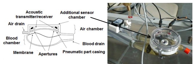
Fig. 9. The POLVAD prosthesis with an additional sensor chamber
