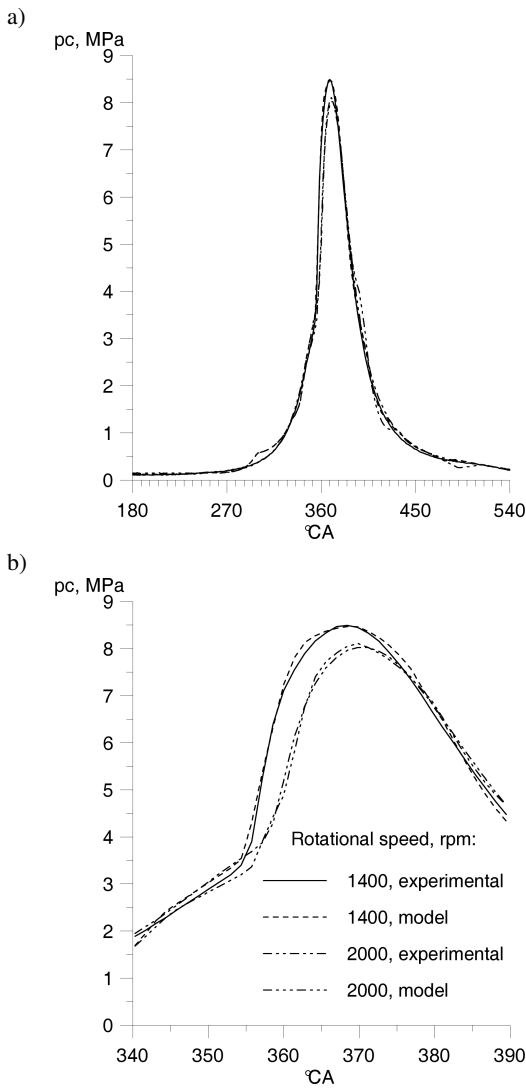
Fig. 5. Comparison of experimental and computed by the fuzzy system (Mamdani model), relationship between cylinder pressure (in engine fueled by diesel oil) and crankshaft rotation angle, for different crankshaft speeds in the range of: a) 180–540°CA, b) 340–390°CA
