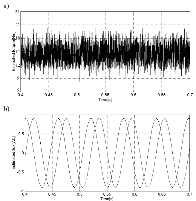
Fig. 7. Estimated steady torque and flux at 500 rpm of classic DTC, T_s = 90 \mu\text{s} , a) estimated torque, b) estimated flux
