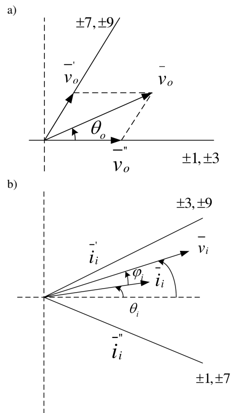
Fig. 4. Synthesis schematic of output voltage vector and input current vector: a) synthesis of output voltage vector b) synthesis input current vector
