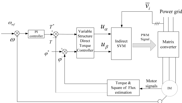
Fig. 3. DTC of induction motor driven by Matrix converter based on variable structure control
