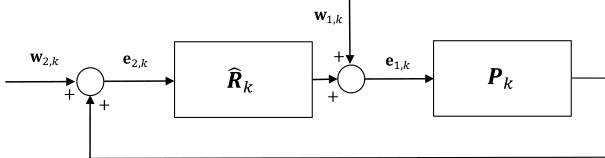
Fig. 2. Block diagram of a closed-loop system
