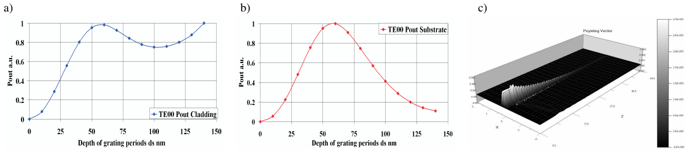
Fig. 3. Optical power rating as a function of the periodical depth d_g of the grating coupler radiated to: a) the light going into environment; b) the substrate; c) Poynting vector along the propagation of light in the grating structure
