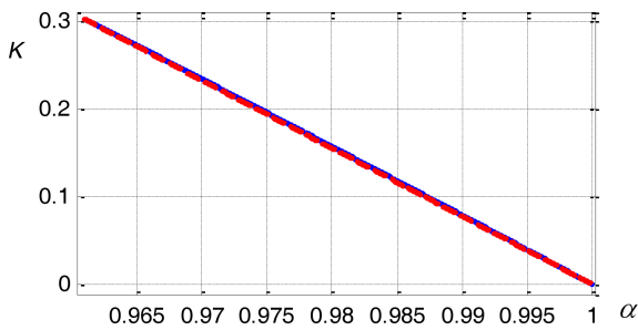
Fig. 11. Nomogram K(\alpha) and the approximation K = 7.8(1 - \alpha)
