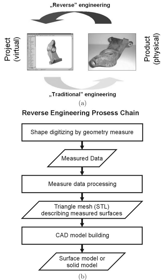
Fig. 14. Reverse engineering idea (Immersion Corp.) (a) and basic operations at creating a 3D CAD model (b)
