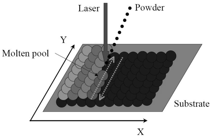
Fig. 9. Operating principle of DLF method (after Ref. 11)
