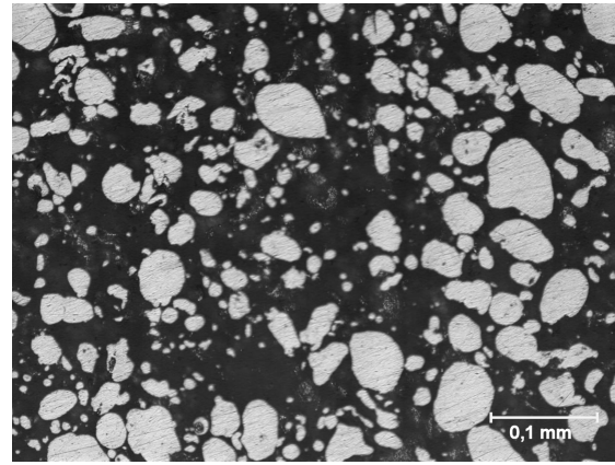
Fig. 25. Microstructure of epoxy resin reinforced with aluminium powder. Volume fraction of powder is 34%, grain size from 2 \mu\text{m} to 0.7 mm. Light microscope (after Ref. 2)
