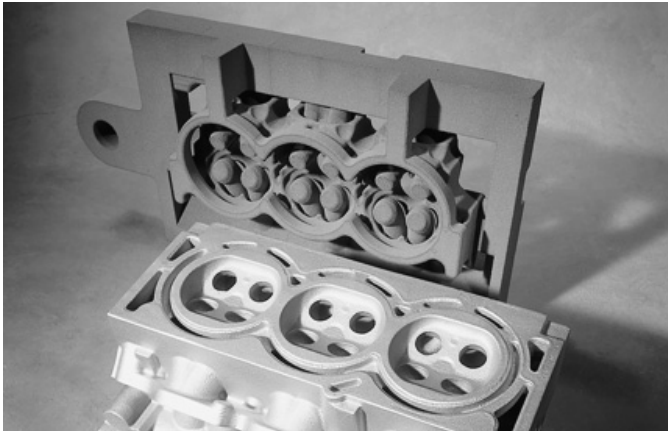
Fig. 8. V6 Cylinder head for 24-valve car engine Integrated sand cores, produced in one piece, for fully functional cast prototypes in AlSi9Cu3 Material: quartz 4.2 Courtesy of: VAW Südalumin and Becker CCC, Germany
