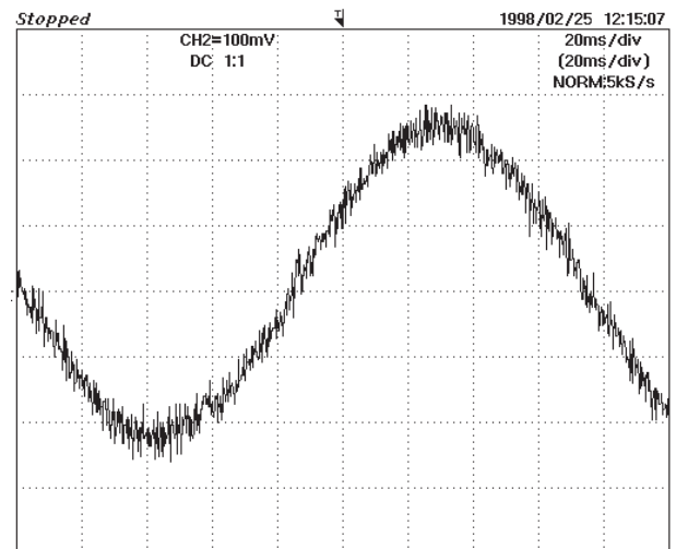
Fig. 31. Measured motor current (8 A/div)
