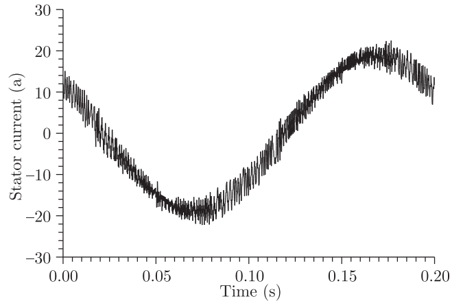
Fig. 29. Basic DTC, \Delta t = 80 \mu s , B_T = 5\% , B_\varphi = 2\% , f_s = 2450 Hz, 100 rpm
