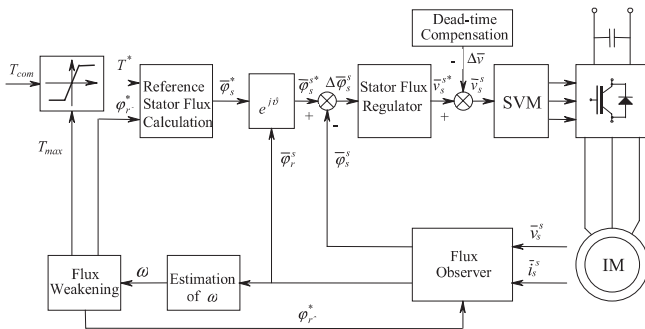
Fig. 18. Block diagram of the scheme based on Stator Flux Vector Control
