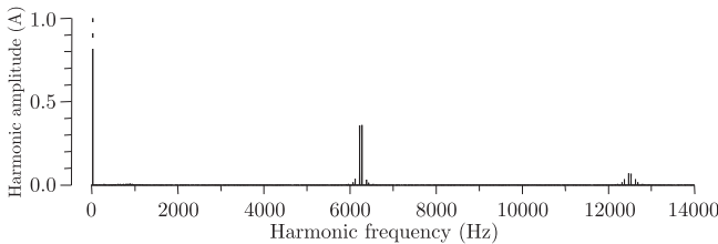
Fig. 33. Stator current harmonic spectrum (DFOC), rated speed, rated torque
