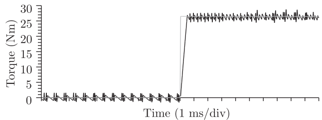
Fig. 36. DTC torque step response
