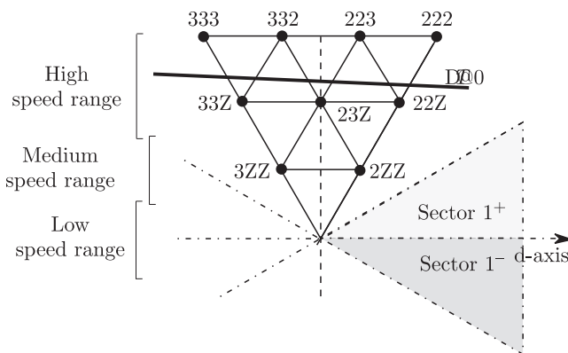
Fig. 28. Representation of the voltage vectors used by the DSVM technique in the high speed range
