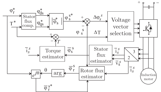
Fig. 16. Block diagram of a DTC scheme with improved stator flux estimator
