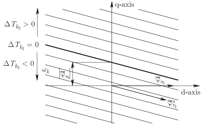
Fig. 8. Diagram of the torque variation \Delta T_{k2}
