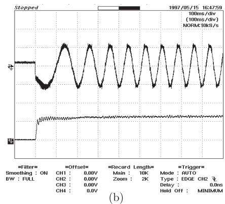
Fig. 17. Torque step response during the start-up, upper trace: phase current, 20 A/div, lower trace: measured torque, 20 Nm/div, (a) pure integrator, (b) improved flux estimator, \tau = 0.01 s
