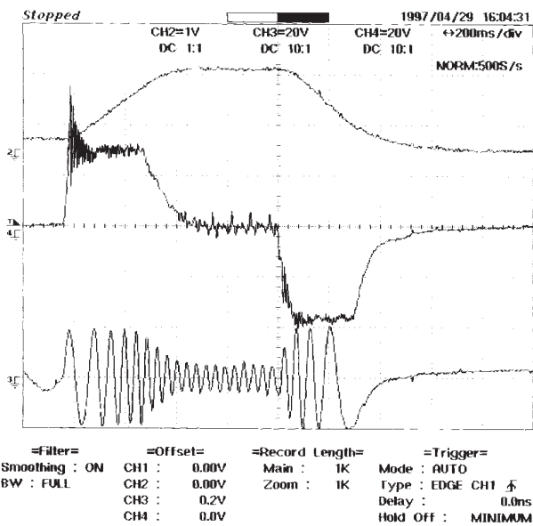
Fig. 25. Transient response of the drive system, top trace: rotor angular speed, middle trace: measured torque, bottom trace: line current, 2 s total acquisition time \Delta R_s = -10\% , \omega = 0 rad/s, \tau = 0.01 s
