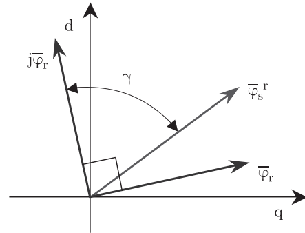
Fig. 3. Stator and rotor flux vectors representation
