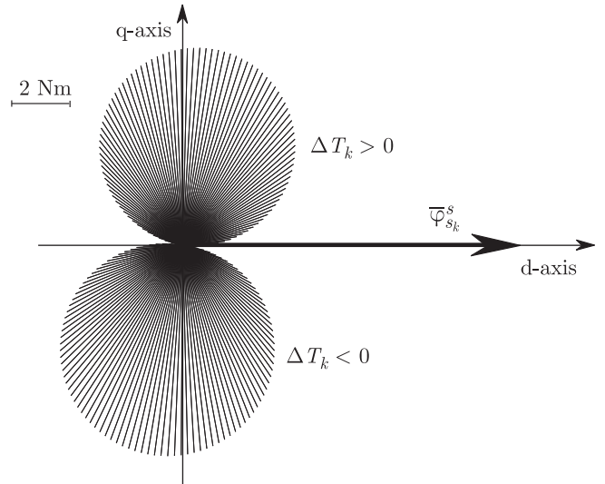
Fig. 9. Torque variations at zero speed (rated torque)
