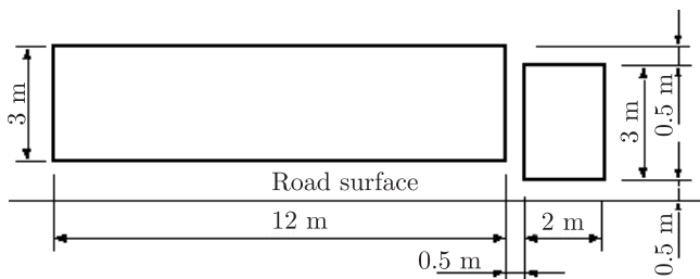
Fig. 4. Lorry geometry
