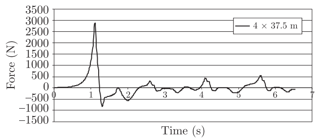
Fig. 23. Vertical force component for 4 lorries at 37.5 m head to head distance
