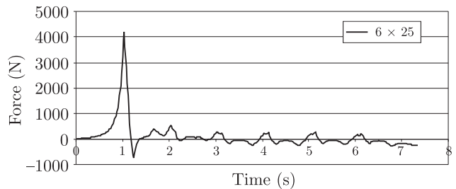
Fig. 24. Vertical force component for 6 lorries at 25 m head to head distance
