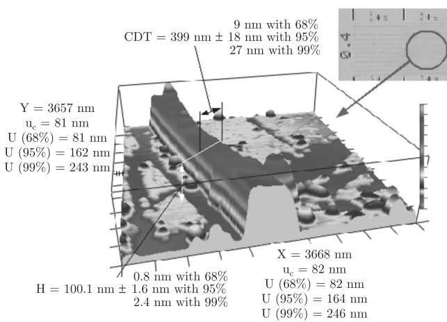
Fig. 5. Topography of the chromium-quartz line structure observed with the calibrated atomic force microscope
