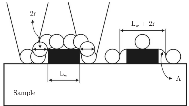
Fig. 6. Measurement of linewidth with the scanning probe microscope
