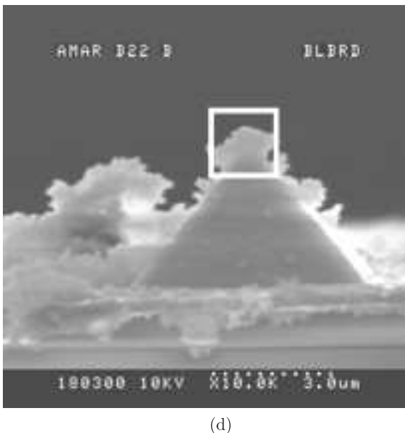
Fig. 8. Characterization of tip shape using SiO 2 nanolines: 3D view of the topography structure a), zoom image of the single nanoline b), crosssection of the tip profile c), SEM image of the tested microprobe d)
