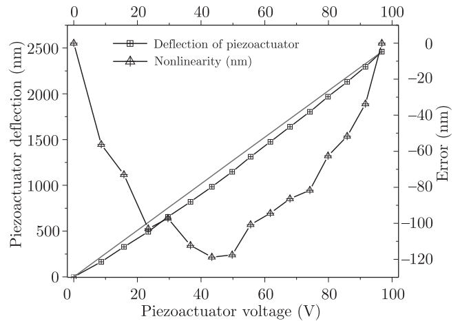
Fig. 1. Piezoelectric actuator deflection measured with the optical fiber interferometer
