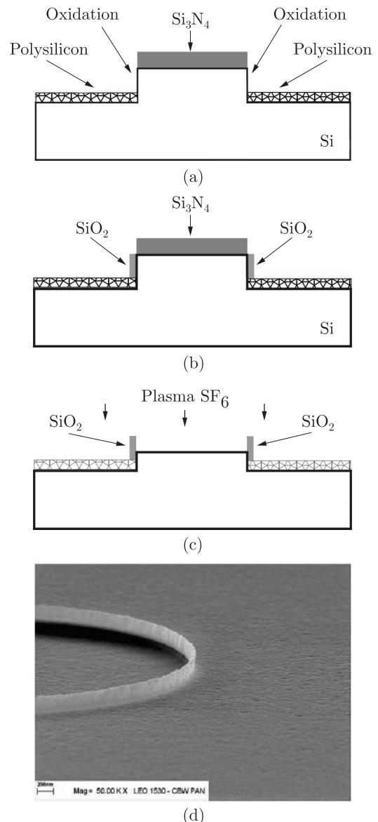
Fig. 7. Fabrication process of the calibration structure for the SPM tip characterization: oxidation of the sidewalls of the Si steps (a), oxidized Si steps before plasma etching of the Si 3 N 4 layer (b), plasma etching of the Si 3 N 4 layer and Si step (c), SEM image of the final device (d)
