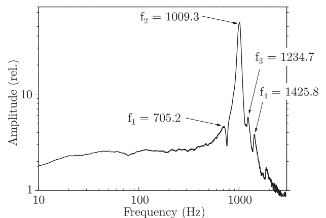
Fig. 3. Piezoelectric actuator deflection as a function of control voltage frequency
