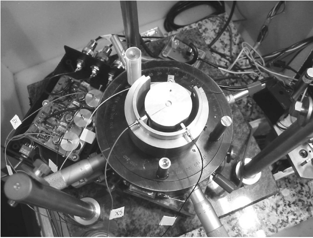
Fig. 4. Scanning Probe Microscopy scanning head with integrated 3 interferometers for measurements of piezoactuator deflection in XYZ directions
