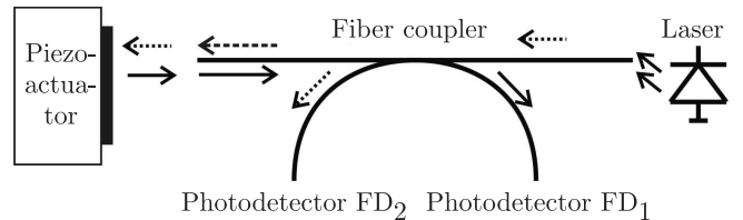
Fig. 2. Schematic diagram of a fiber optical interferometer displacement sensor
