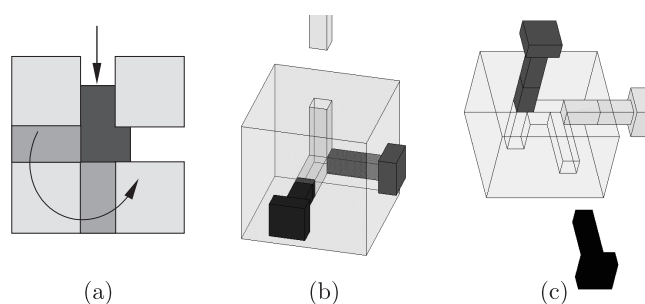
Fig. 6. Multi-punch ECAP procedure: with rotating die (a), with multi-pass channels (b), with one-pass channels (c)
