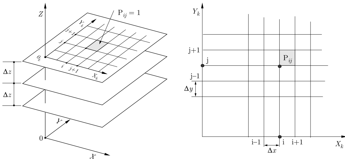
Fig. 1. A general scheme for binary representation and evaluation of manipulator workspace
